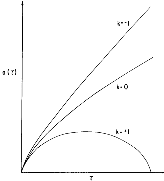
Fig. 5.4. The dynamics of radiation-filled Robertson-Walker universes.
