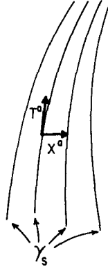
Fig. 3.5. A one-parameter family of geodesics \gamma_s , with tangent T^a and deviation vector X^a .
