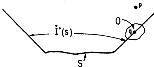
Fig. 8.3. A spacetime diagram showing a set S and the boundary of its future, I^+(S) (see theorem 8.1.3).
