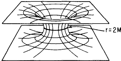
Fig. 6.10. The spatial geometry of the hypersurface t = 0 of the Schwarzschild spacetime, shown as it would look if it were embedded in flat space. (One dimension is suppressed, i.e., the topology of the hypersurface is \mathbb{R} \times S^2 , not \mathbb{R} \times S^1 , so each circle—such as the one shown at r = 2M —really represents a two-sphere.) The portion of the surface lying above the “throat” at r = 2M in the figure corresponds to the portion lying in region I of Figure 6.9; the portion below r = 2M lies in region IV of Figure 6.9.
