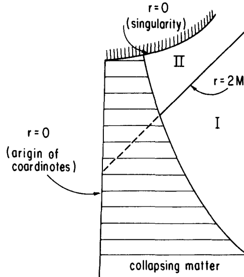
Fig. 6.11. The spacetime resulting from the complete gravitational collapse of a spherical body. All of regions III and IV of the extended Schwarzschild spacetime (Fig. 6.9) are "covered up" by the collapsing matter. However, (part of) the black hole region II is produced.
