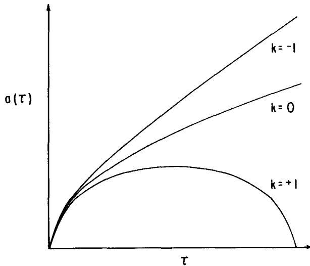
Fig. 5.3. The dynamics of dust-filled Robertson-Walker universes.
