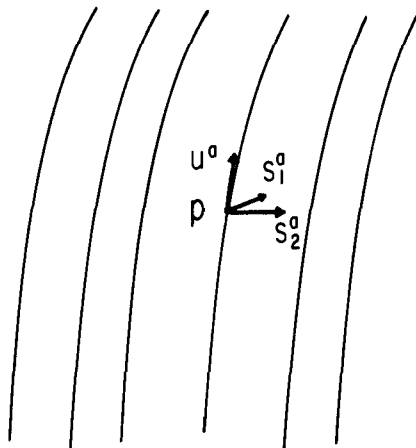
Fig. 5.2. The world lines of isotropic observers in spacetime. By definition of isotropy, for any two vectors s_1^a, s_2^a at p which are orthogonal to u^a , there exists an isometry of the spacetime which leaves p fixed and rotates s_1^a into s_2^a .
